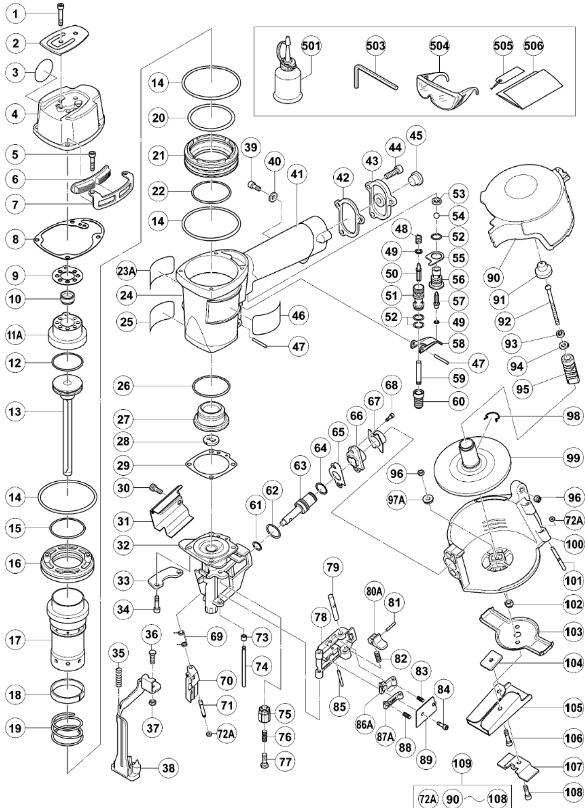
Side Load Magazine Ass'y
